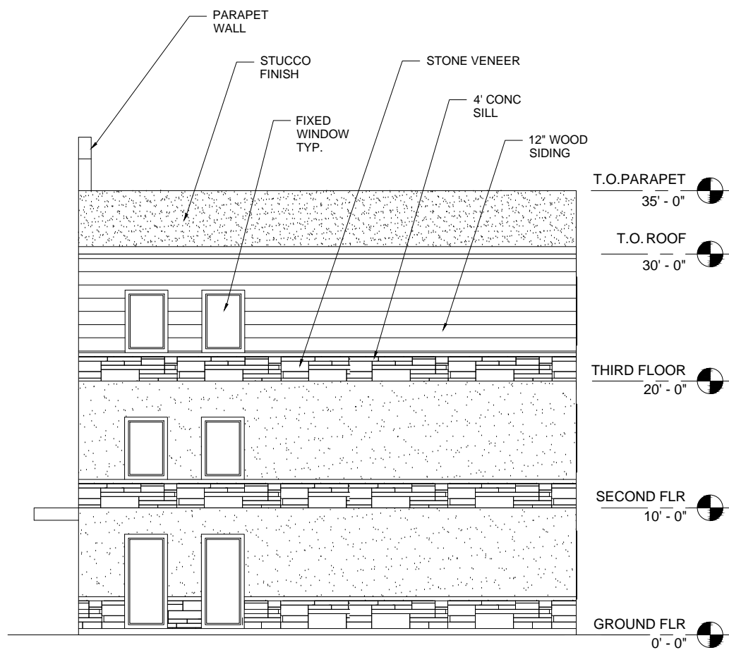
2 RIGHT SIDE ELEVATION A-6 3/32" = 1'-0"
