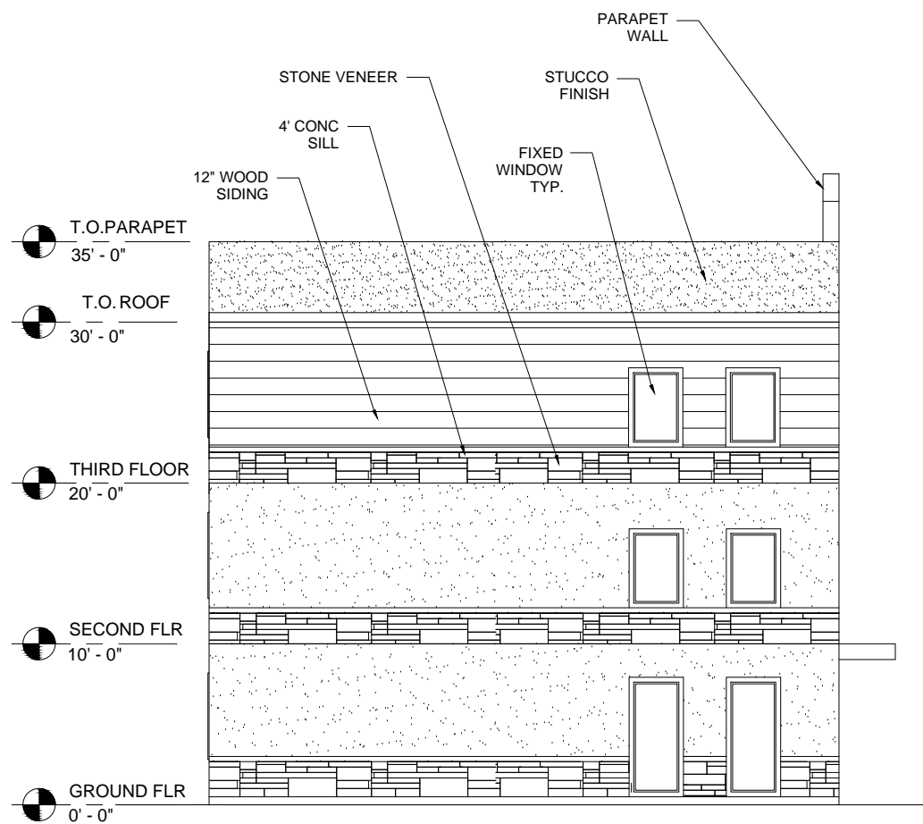
1 LEFT SIDE ELEVATION A-6 3/32" = 1'-0"
