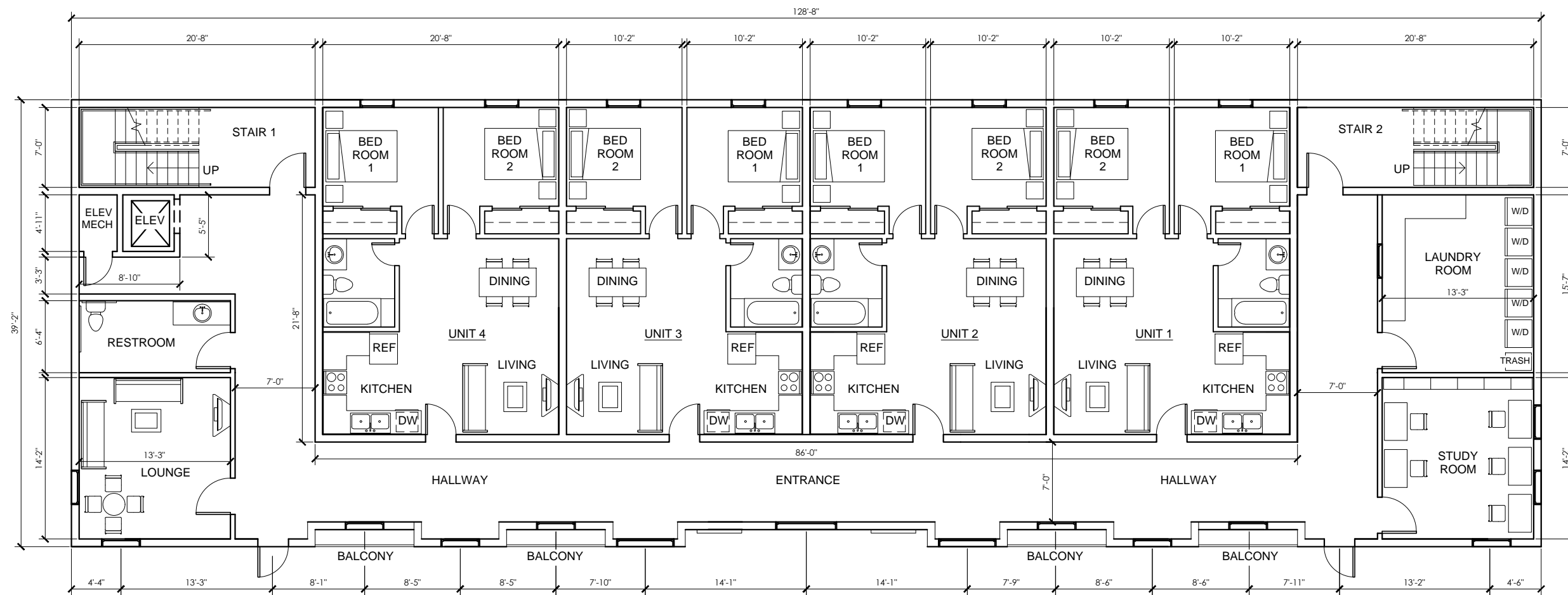
1 2ND & 3RD FLOOR PLAN A-3 3/32" = 1'-0"
