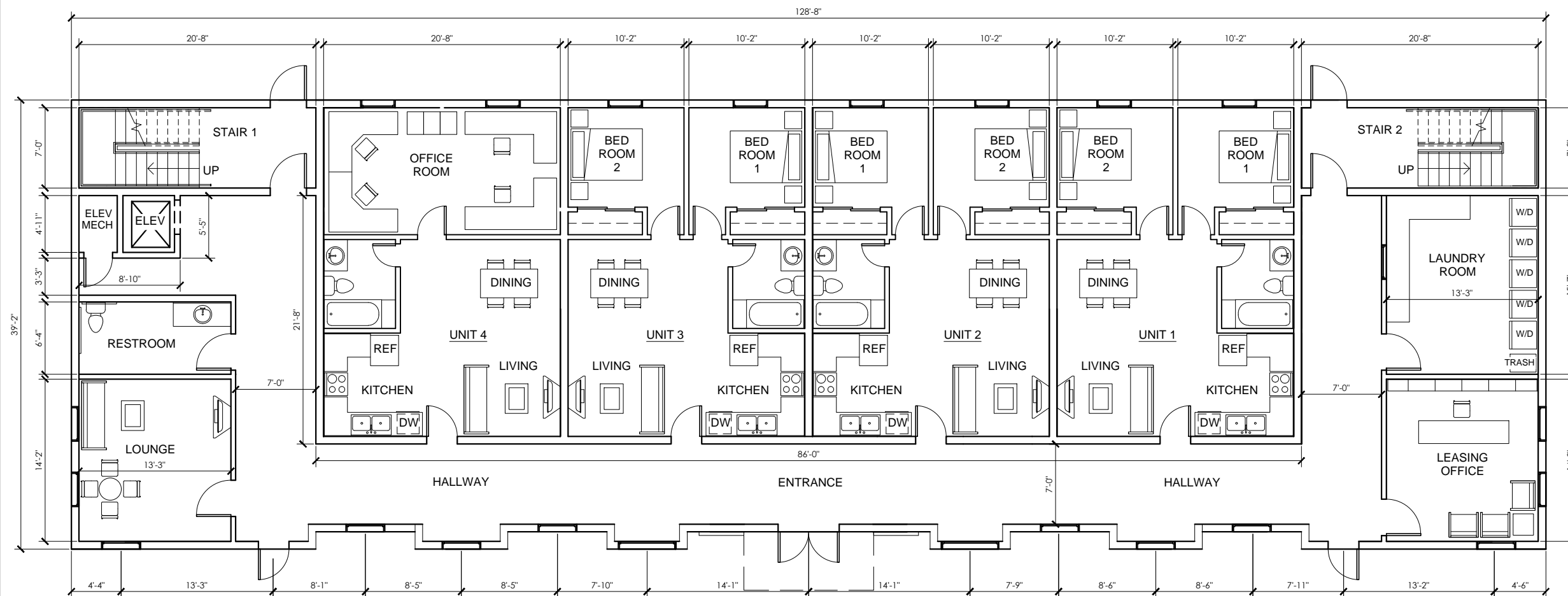
1 GROUND FLOOR PLAN A-2 3/32" = 1'-0"
